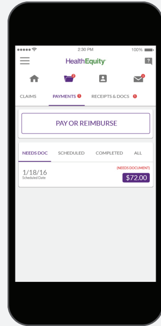
PAYMENTS SCREEN
